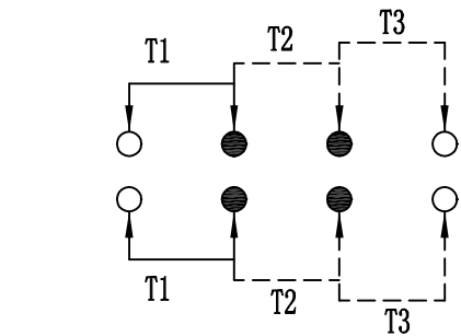
SCHEMATIC (NON-SHORTING)
